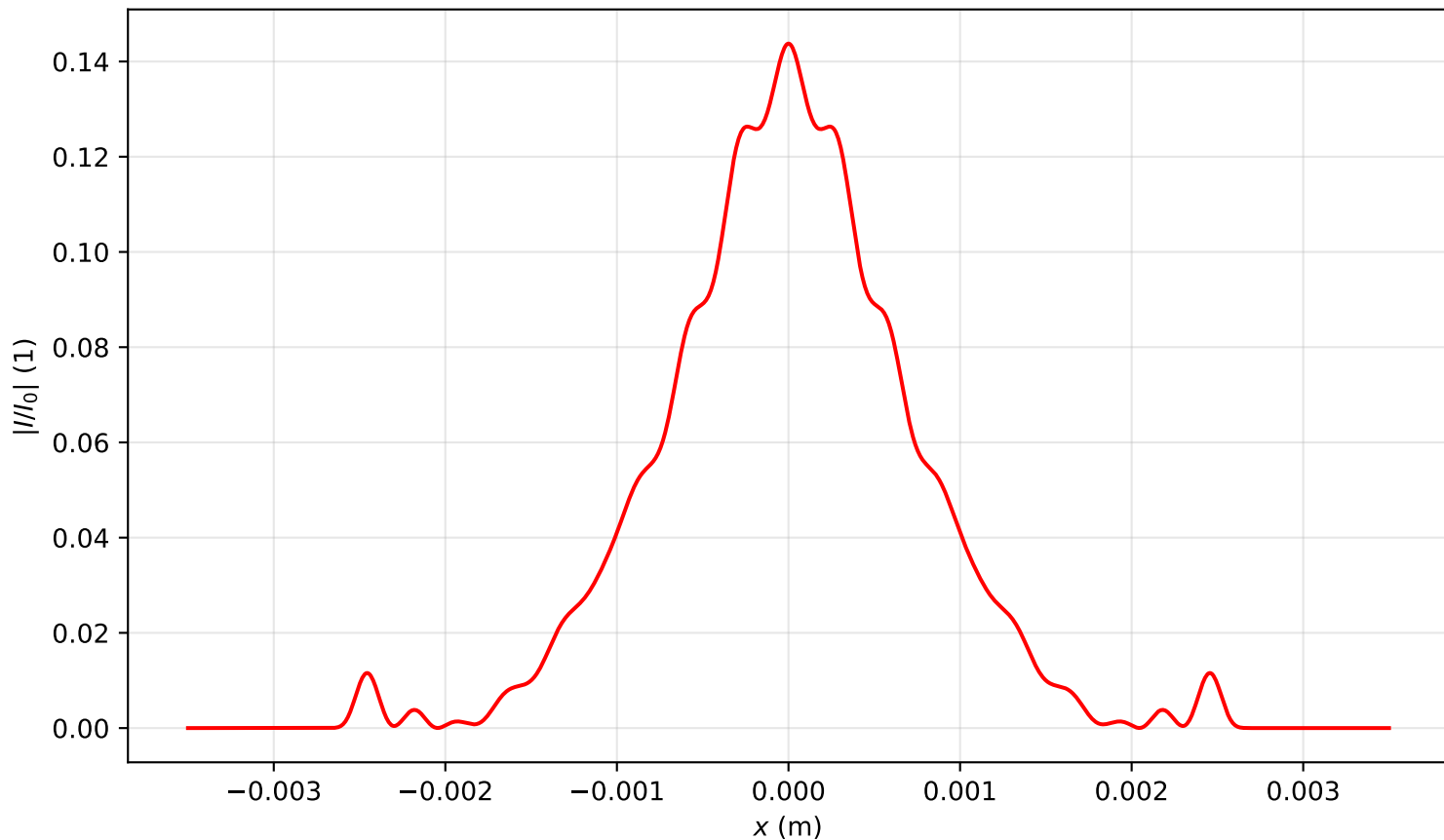
Intensity profile I(x, y = 0, z = 2.070)/I_0 , P_{in}=2.0P_{cr} , artificial time
